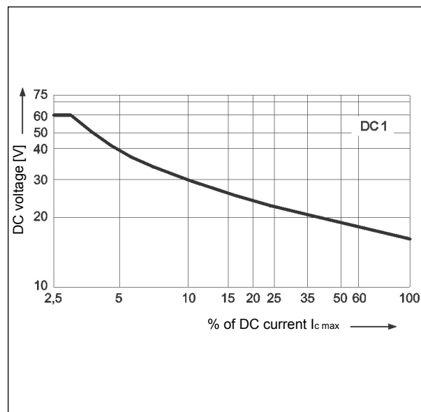
Max. DC resistive load breaking capacity Fig. 1
